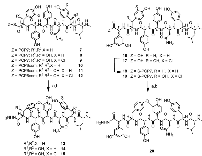
Scheme 2. In vitro conversion of linear hexapeptides ( 7–12 ) to monocyclic peptides ( 13–15 ) by OxyB, and linear heptapeptides ( 16–19 ) and only observed cross-linked product ( 20 ). Reagents: a) OxyB, spFd, ecoFldR , NADPH, G6P, G6P-DH, air, 1 h, 30 °C; b) hydrazine, 30 min, 30 °C.
