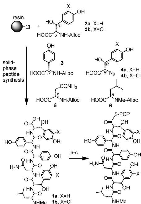
Scheme 1. Synthesis of the hexapeptide substrates. For the synthesis of amino acids 2–6 , and the solid-phase synthesis of 1a and 1b , see the Supporting Information. Reagents: a) N -methylmorpholine (1.2 equiv), PyBOP (1.2 equiv), PhSH (2.4 equiv), DMF, 30 min, RT; b) CoASH (4.0 equiv), phosphate buffer (50 mM, pH 7.5)-DMF (2:1), 1 h, RT; c) apo -PCP domain, Sfp from B. subtilis , 30 min, 37 °C. Alloc = allyloxycarbonyl.
