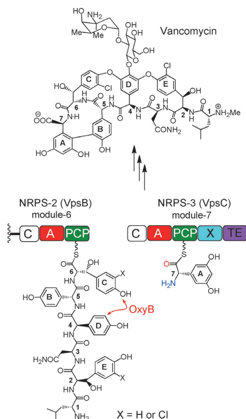
Figure 1. Key steps of backbone assembly during vancomycin and balhimycin biosynthesis (vancomycin and balhimycin share the same aglycone). Shown is the predicted domain organization of modules 6 and 7, in the vancomycin NRPS subunit 2 (VpsB) and 3 (VpsC) (C = condensation domain, A = adenylation domain, PCP = peptide carrier protein domain, TE = thioesterase domain, X = domain of unknown function). The hexapeptide-S-PCP thioester intermediate shown should be cross-linked by OxyB before addition of the last amino acid (Dpg 7 ) by module 7.
