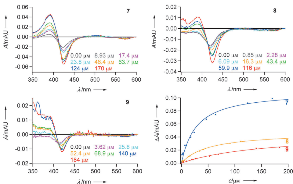
Figure 3. Difference UV/Vis spectra from binding of substrates 7 , 8 , and 9 to OxyB, and the dependence of spectral changes on the peptide concentration c .
