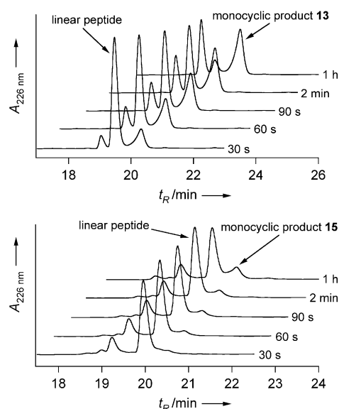
Figure 2. HPLC chromatograms showing typical time courses of product formation ( 13 and 15 ) from substrates 7 (top) and 9 (bottom), respectively (Supporting Information, Figure S11). The peak retention time ( t_R ) and peak absorbance at 226 nm are shown.
